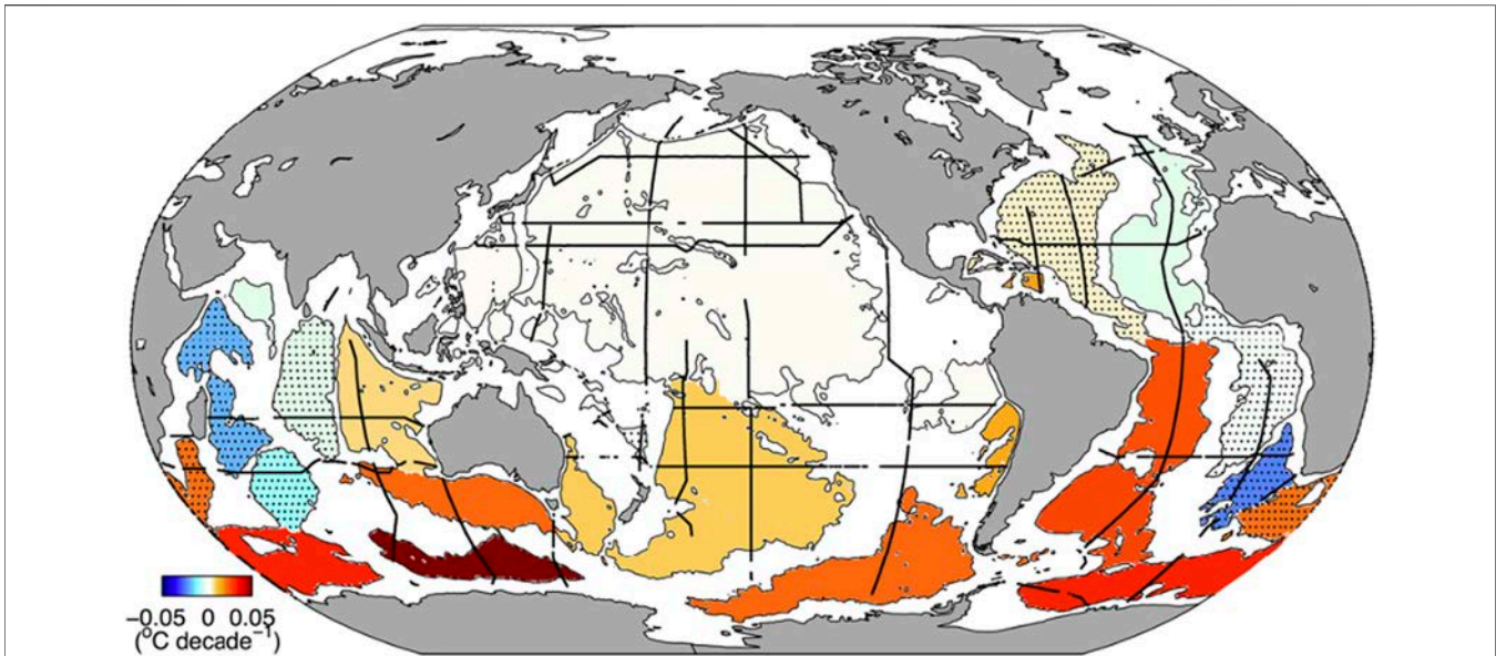
FIGURE 6 | Deep basin (thin solid lines) average warming rates below 4,000 m from the 1990s to the 2000s ( ^{\circ}\text{C decade}^{-1} , colorbar) based on data from Purkey and Johnson (2010). Estimates are based on data from decadal repeats of hydrographic sections (thick solid lines) first occupied during the World Ocean Circulation Experiment (WOCE) (King et al., 2001) and subsequently by GO-SHIP (Talley et al., 2016). Stippled basins have average warming rates that are not statistically significantly different from zero at 95% confidence. Permission obtained for use of figure.
