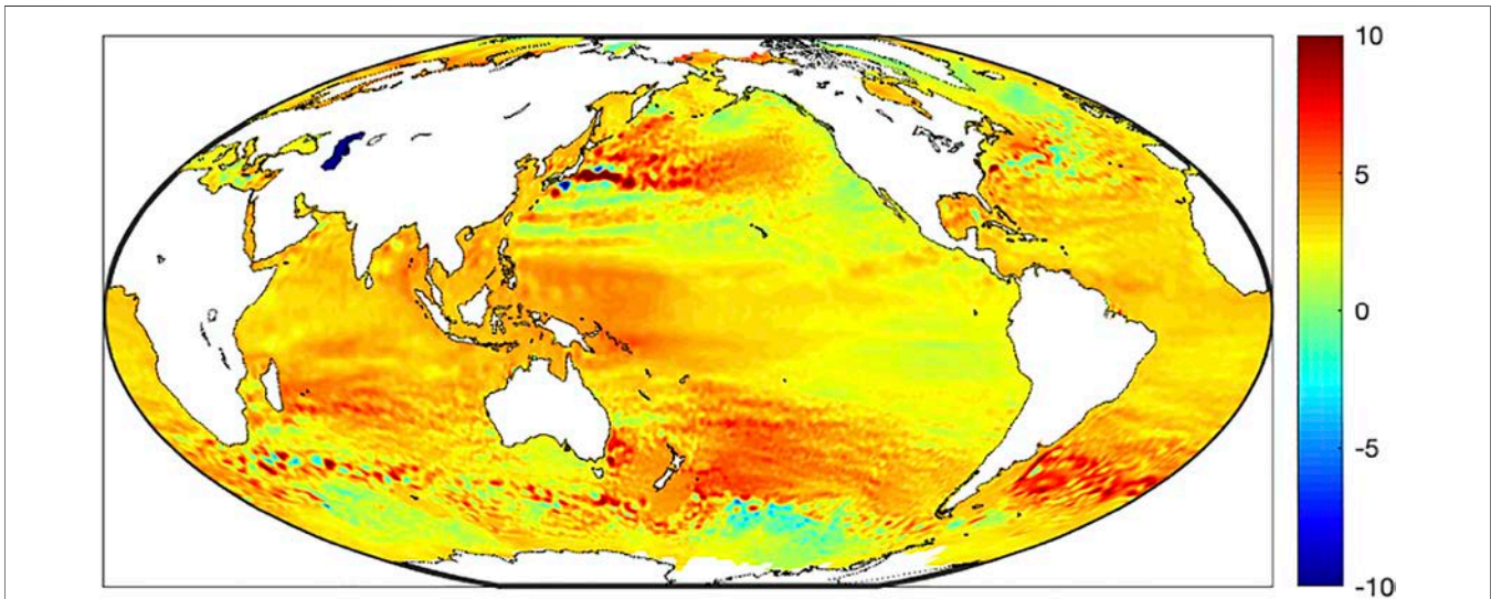
FIGURE 7 | Mean sea level trend (mm/y; January 1993–October 2019) from multi-mission satellite altimetry (data source: AVISO).
